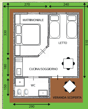
PIANTINA BUNGALOW
